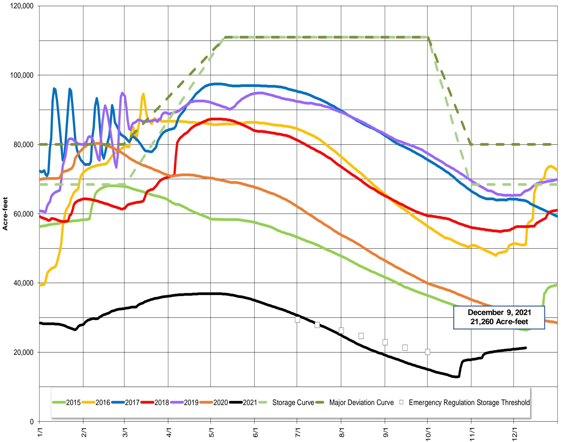
Lake Mendocino Storage 2015 - 2021 and Storage Curve
